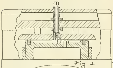
DISCONNECTED VALVE WITH LOCK BOLT.
